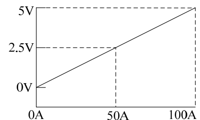
输出曲线对应图 Output Curve Diagram
