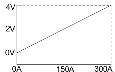
输出曲线对应图 Output Curve Diagram
