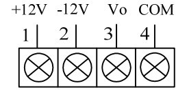
接线图 Connecting Diagram
